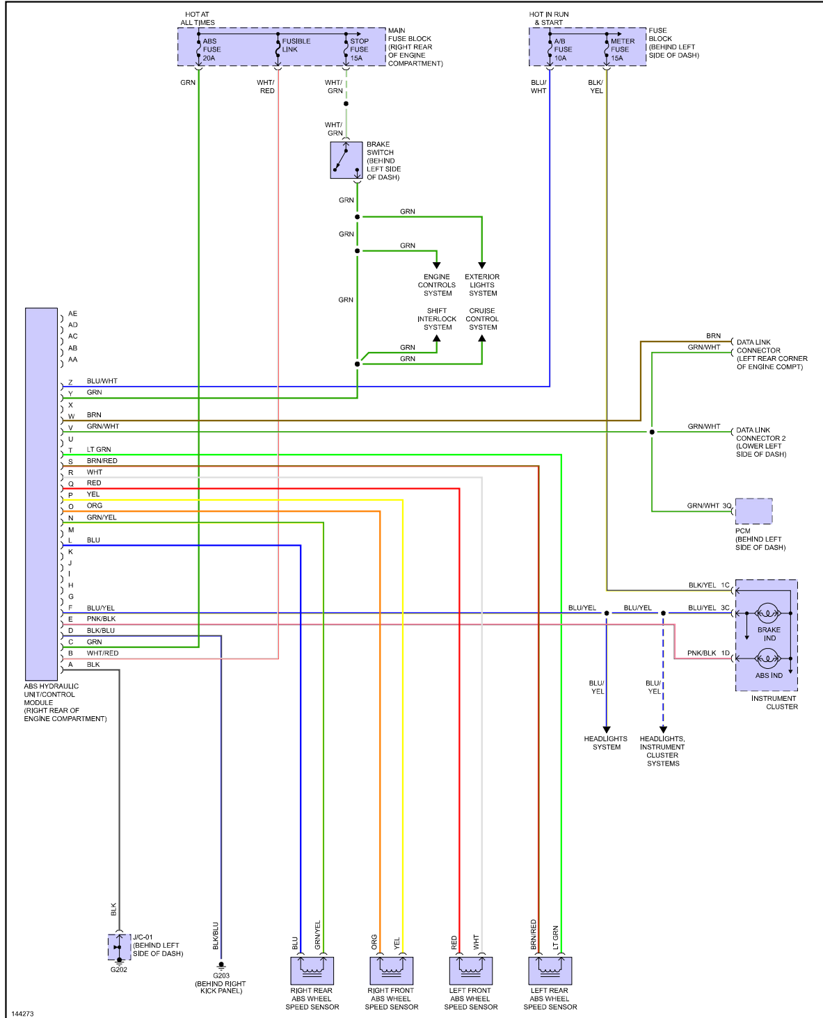
Fig 1: Anti-lock Brake Circuits
