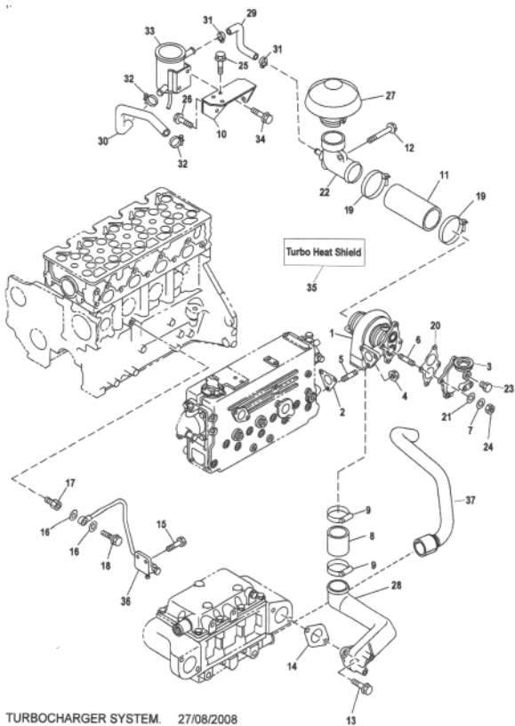
TURBOCHARGER SYSTEM. 27/08/2008
