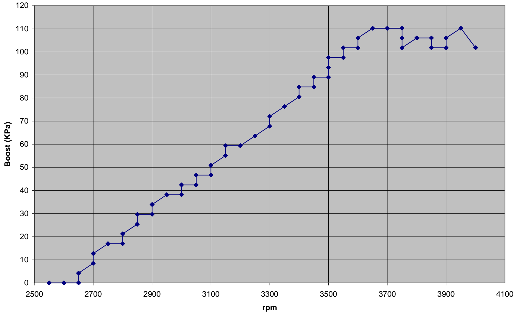
Boost response
