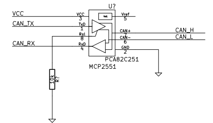
CAN transceiver
