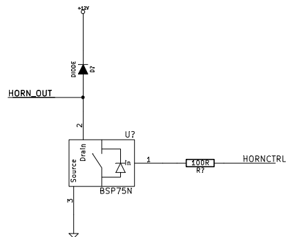
Horn Relay output driver
