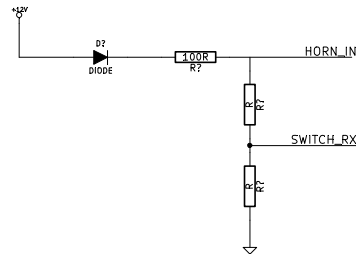
One wire coms RX from steering wheel switches.
