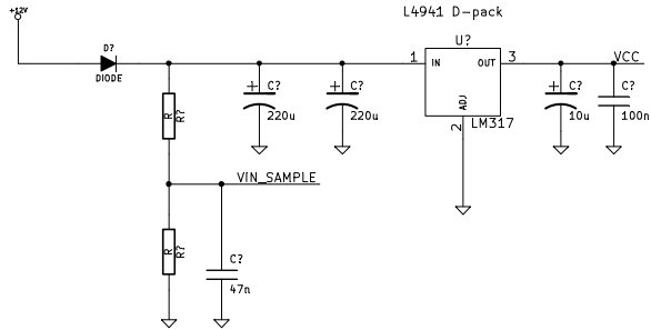
Regulator and low voltage shutdown sampling
